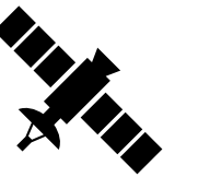
Voyager 1 23 billion KM
